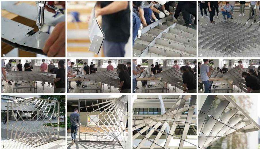
Figure 6. A-D: Prefabrication. E-H: Elastic formation. I-L: Completed module.
