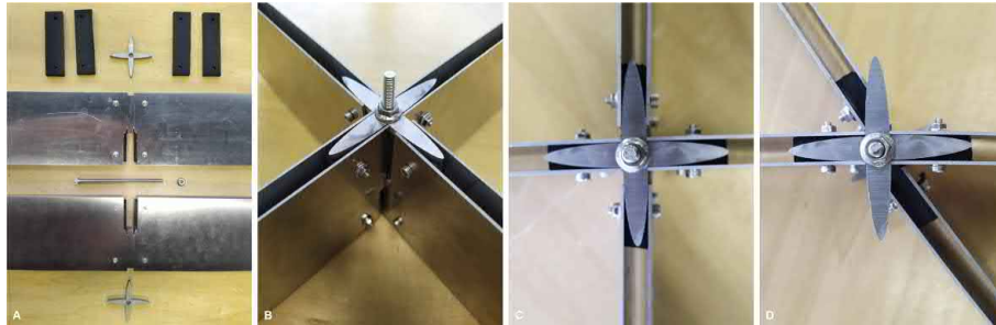
Figure 4. Composite joint system from two 1.5mm stainless steel strips with 8mm rubber inlays (A). The joints are designed to allow up to +30^\circ rotation freedom during assembly (D) and lock at 90 degrees once the rounded star-washers are fixed (B, C).
